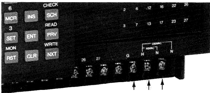
Figure 3.4 POWER CONNECTIONS
