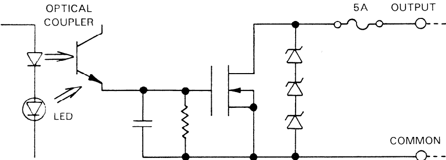
Figure 6.30 WIRING OF 24 V dc 2 AMP SINK/SOURCE OUTPUT
