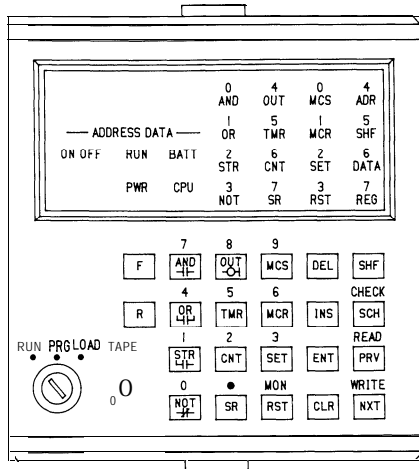
Figure 5.2 PROGRAMMER
