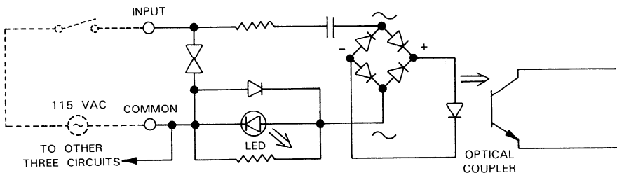
SAMPLE INPUT CIRCUIT
